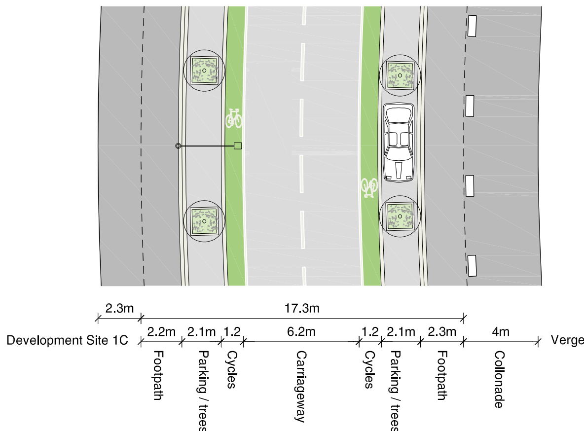
7 DA3.101 BRODIE SPARK DRIVE SOUTH PART PLAN
